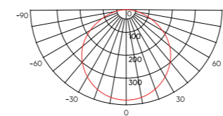
LM-LED/3KK
